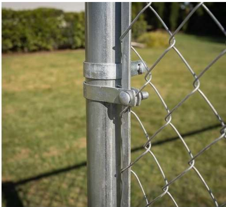
SIDE VIEW (POST)
